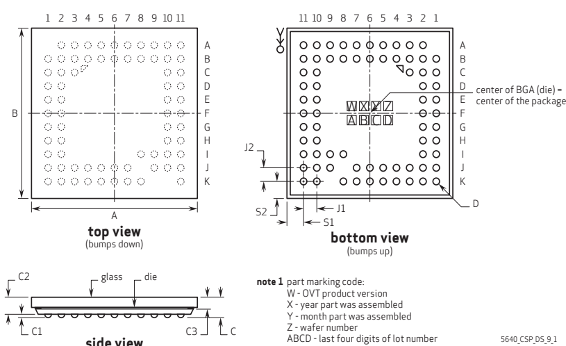
figure 9-1 package specifications
